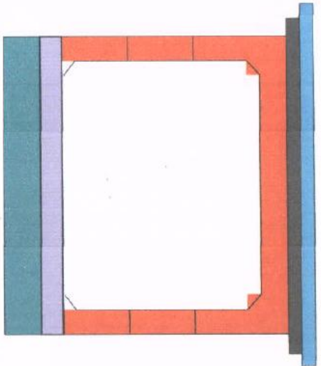
BOX CULVERT 55+820
