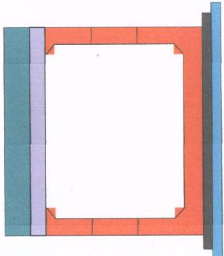
BOX CULVERT 53+900
